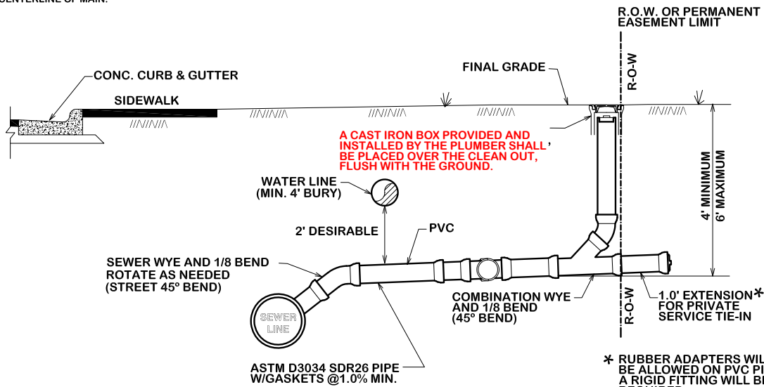
ELEVATION VIEW
