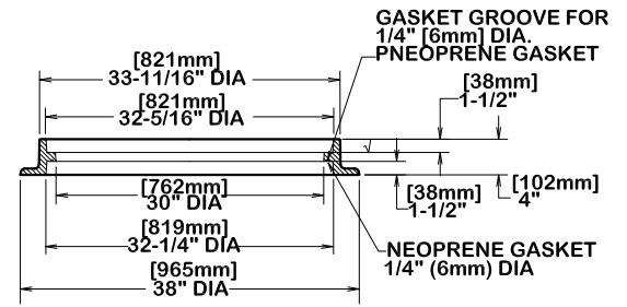
FRAME SECTION
