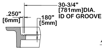
MACHINE GROOVE DETAIL
