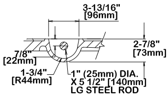
PICKBAR DETAIL
