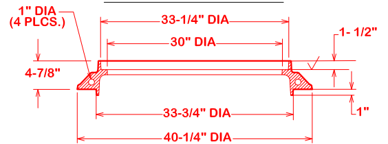
FRAME SECTION
