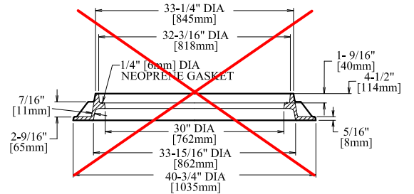
FRAME SECTION
