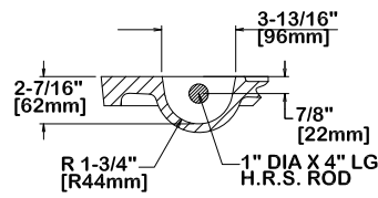
PICKBAR DETAIL
