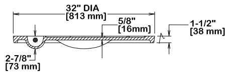
COVER SECTION
