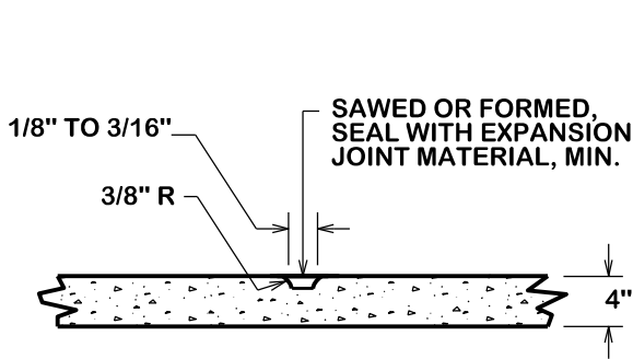
SIDEWALK CONTRACTION JOINT
