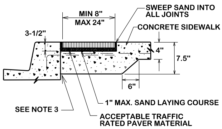
SIDEWALK PAVER SECTION
