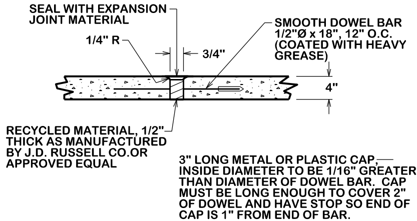
SIDEWALK CONTRACTION JOINT
