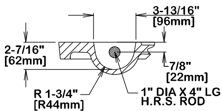
PICKBAR DETAIL
