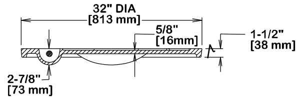
COVER SECTION
