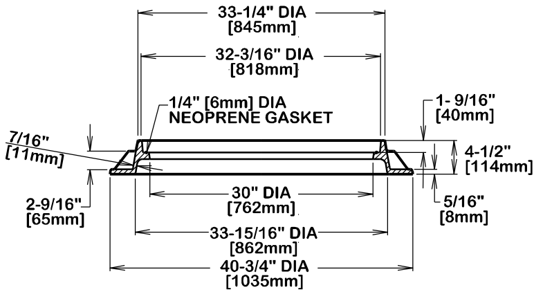
FRAME SECTION
