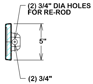
CROSS SECTION
